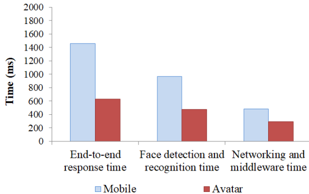
Figure 5: End-to-end response time of LostChild app when major computation workload is at the mobile and avatar, respectively
