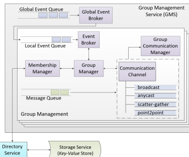
Figure 4: Group Management Service
