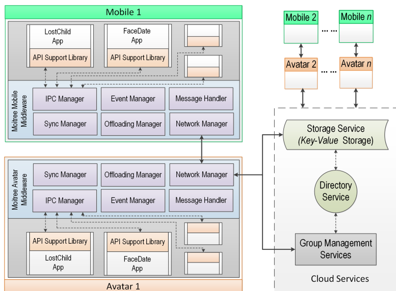
Figure 2: Components of the Moitree Middleware
