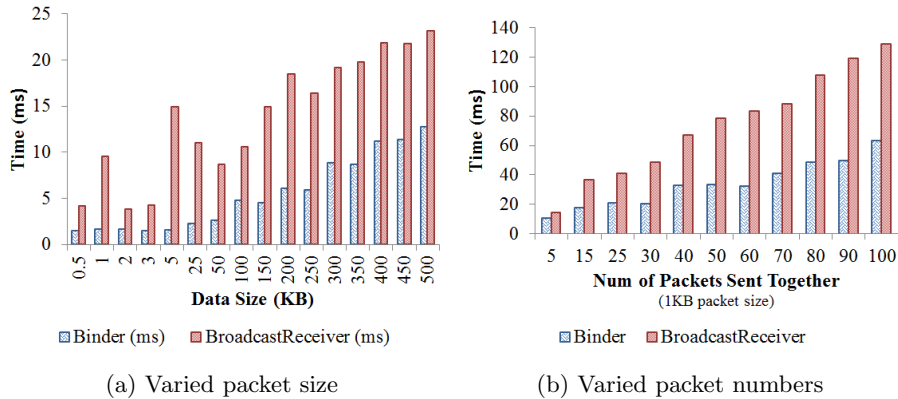
Figure 9: IPC latency of BroadcastReceiver-based mechanism and Binder-based mechanism
