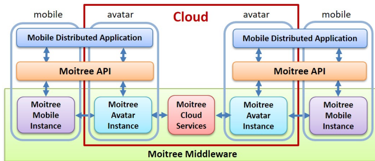
Figure 1: Execution of distributed apps facilitated by Moitree
