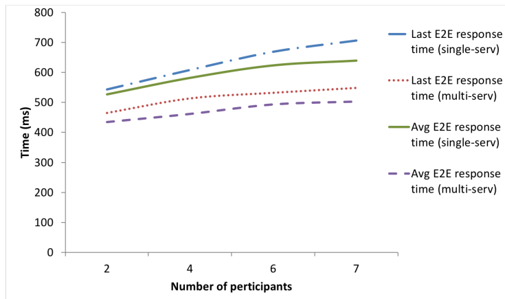
Figure 6: End-to-end response time of LostChild app with an increasing number of participants. The curves marked with “single-serv” are obtained with all participant avatars running on the same server; and the curves marked with “multi-serv” are obtained with each participant avatar running on a different server.
