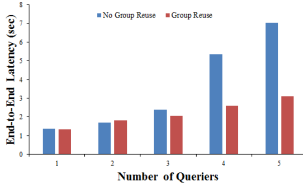
Figure 8: End-to-end response time for FaceDate app with an increasing number of queriers and one positive responder
