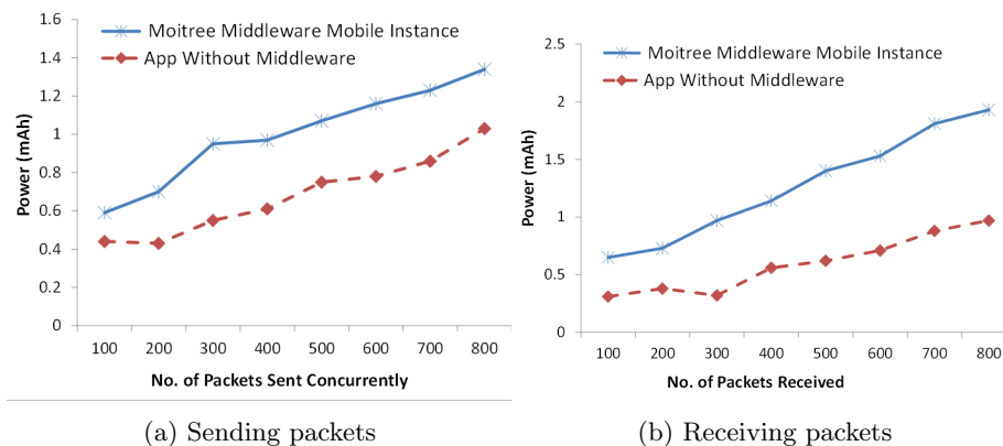
Figure 13: Power consumption overhead caused by sending and receiving data with a Moitree-based app compared to an app without Moitree support. The packet size is 50KB.
