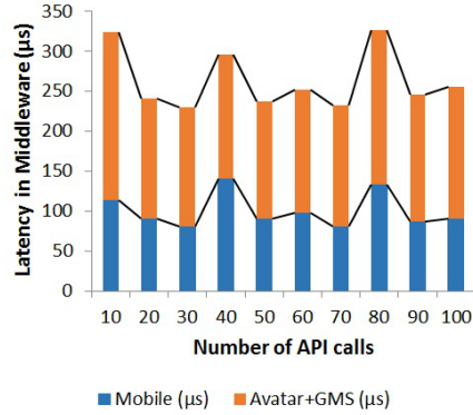
Figure 12: Average processing time for API calls in Moitree on mobile and avatar (no network communication)
