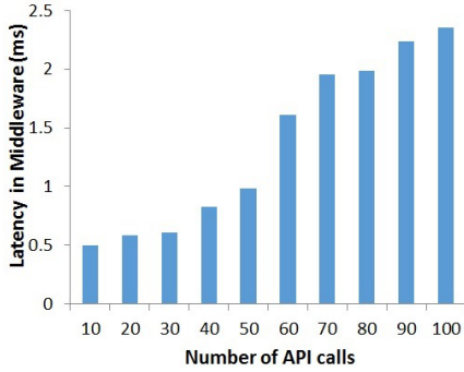
Figure 10: Network serialization and deserialization delay
