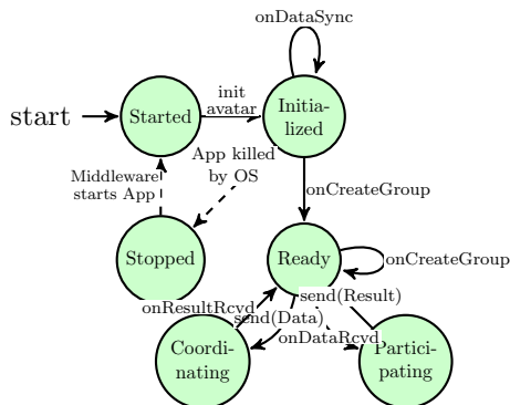
Figure 3: App State Diagram
