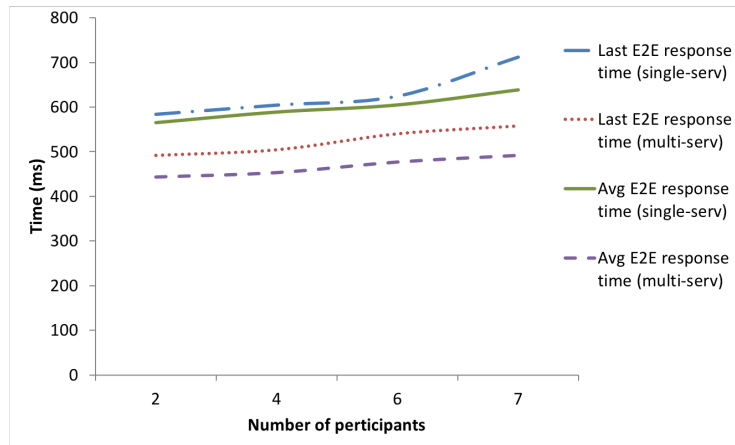
Figure 7: End-to-end response time of FaceDate app with an increasing number of participants.
