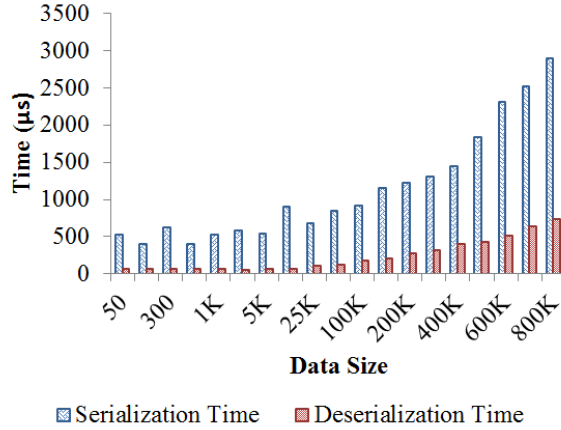
Figure 10: Network serialization and deserialization delay
