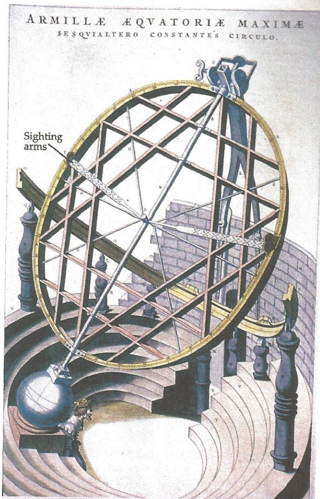
Figure 2. The equatorial armillary , Tycho's most impressive instrument, completed in 1585. The tilted axis running through the large (2.7-m wide) circle is parallel with Earth's axis. The circle is calibrated with 90^\circ at the poles and 0^\circ at the midpoint of its circumference. Two sighting arms establish the declination, the angular distance (north or south) of a star from the equator. Tycho could use one sighting arm to read the declination of a star or planet and then, in less than a minute's time, rotate the circle 180^\circ about the tilted axis to make a second independent determination with the other arm. (Published in 1662 and based on Tycho's original version, this illustration is by Willem Blaeu, a former assistant at Tycho's Hven observatory.)
