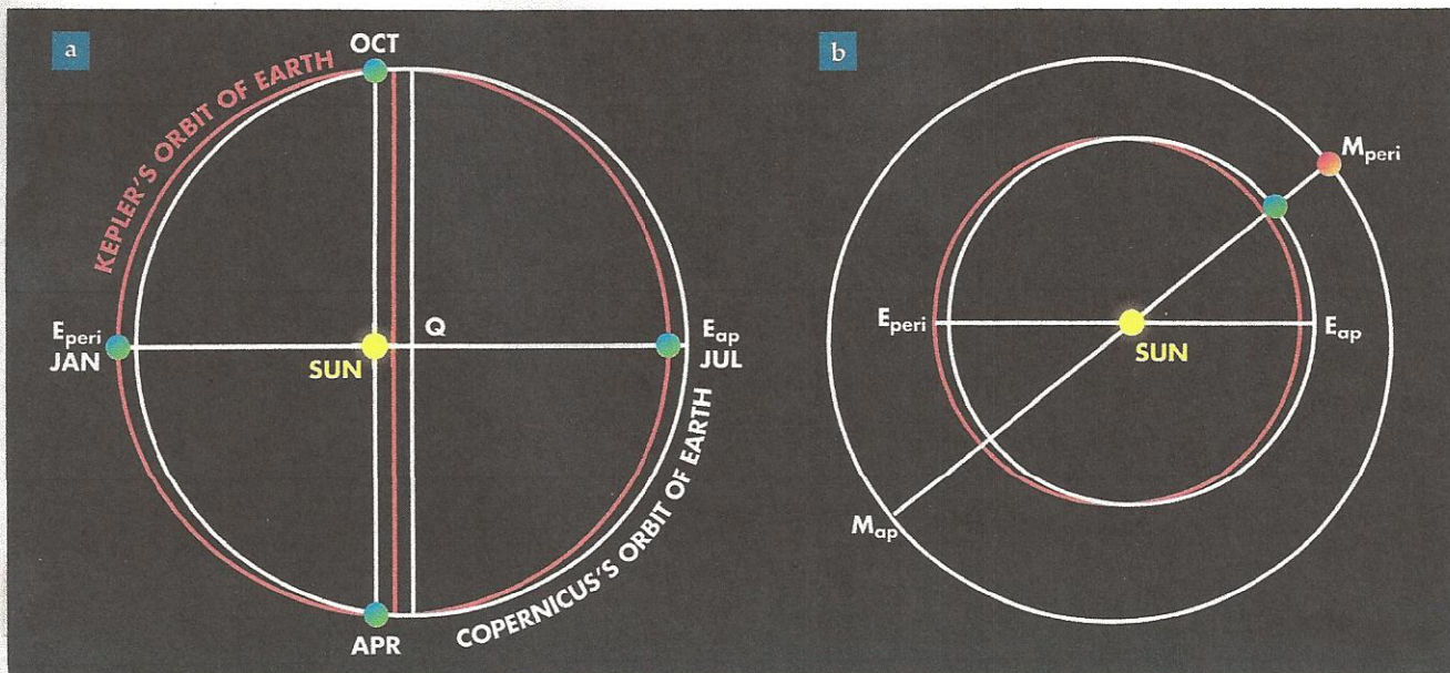
Figure 4. (a) In Nicolaus Copernicus's system, Earth (green) moves uniformly around a point Q (called an equant), the center of its eccentric orbit, from aphelion E_{ap} to perihelion E_{peri} and back. Because the observed quadrant from January to April has a shorter part of the circumference than the quadrant from April to July, the Sun appears to move more quickly during the Northern Hemisphere's winter than during its summer; hence winter is shorter than summer. But because Johannes Kepler believed that Earth should actually move faster when it is nearer the Sun, he bisected the eccentricity and thereby shifted Earth to a less eccentric orbit (red). In Kepler's system, half the Sun's apparent nonuniform motion is caused by the eccentric position of the Sun, and half is caused by the actual nonuniform motion of Earth. (b) The orbits of Mars (M, red) and Earth (E, green) are shown to scale, with Mars at its perihelion making its closest approach to Earth at the time of the great Martian catastrophe. When Kepler bisected the eccentricity of Earth's orbit, the orbit's center slipped along the apsidal line away from the direction of its aphelion. That repositioned Earth just enough to eliminate the major errors in the observed longitude of Mars. In both diagrams the eccentricity of Earth's orbit is greatly exaggerated for clarity.
