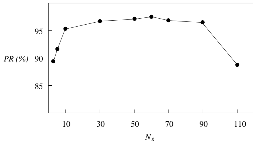
Figure 3: Impact of N_g in the BNN classifier.
