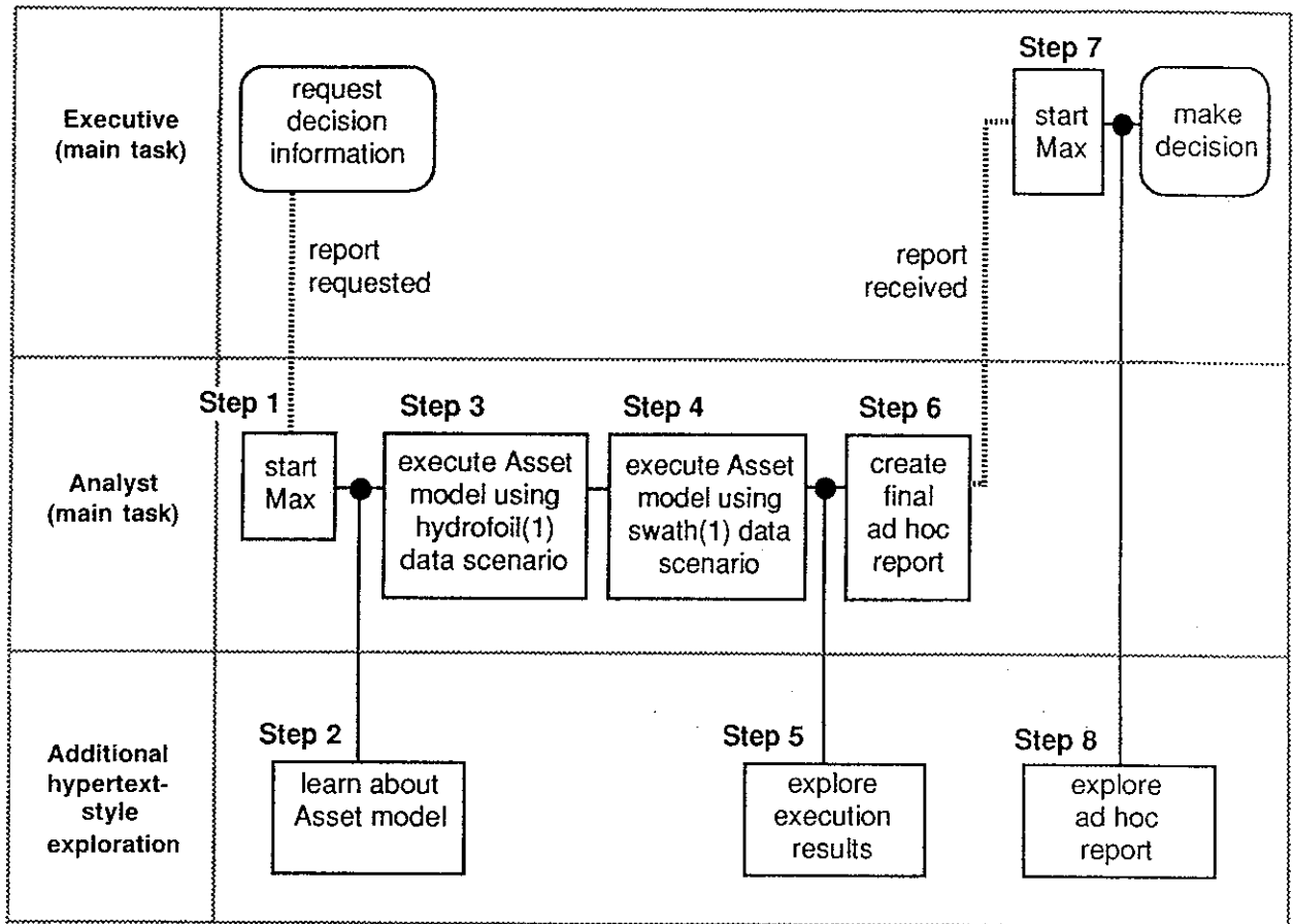
Figure 4. An Analysis Task Supported by Max
