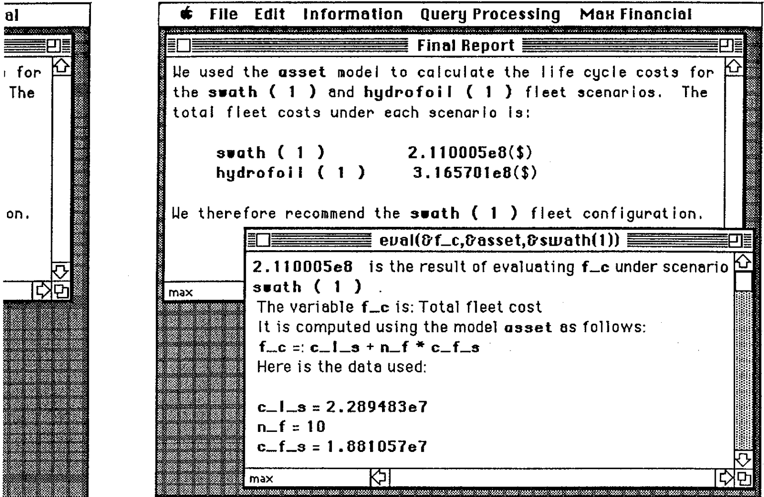
Figure 8. System Generated Report Explaining the SWATH Fleet Cost Number in the Analyst's Final Report
