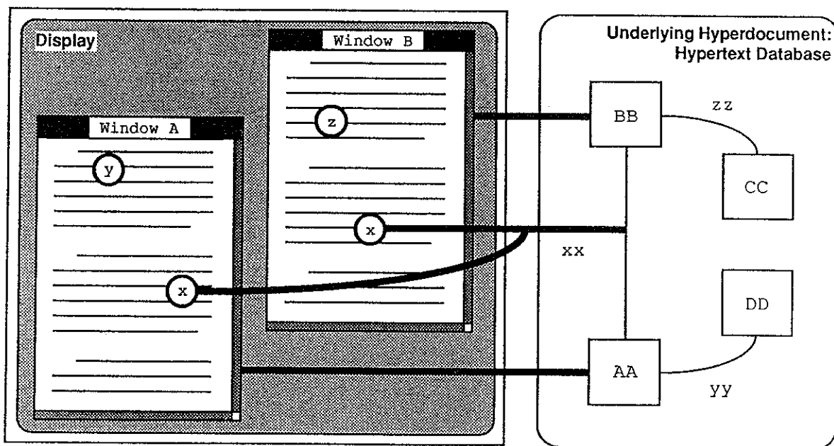
Figure 1. Central Hypertext Concept
