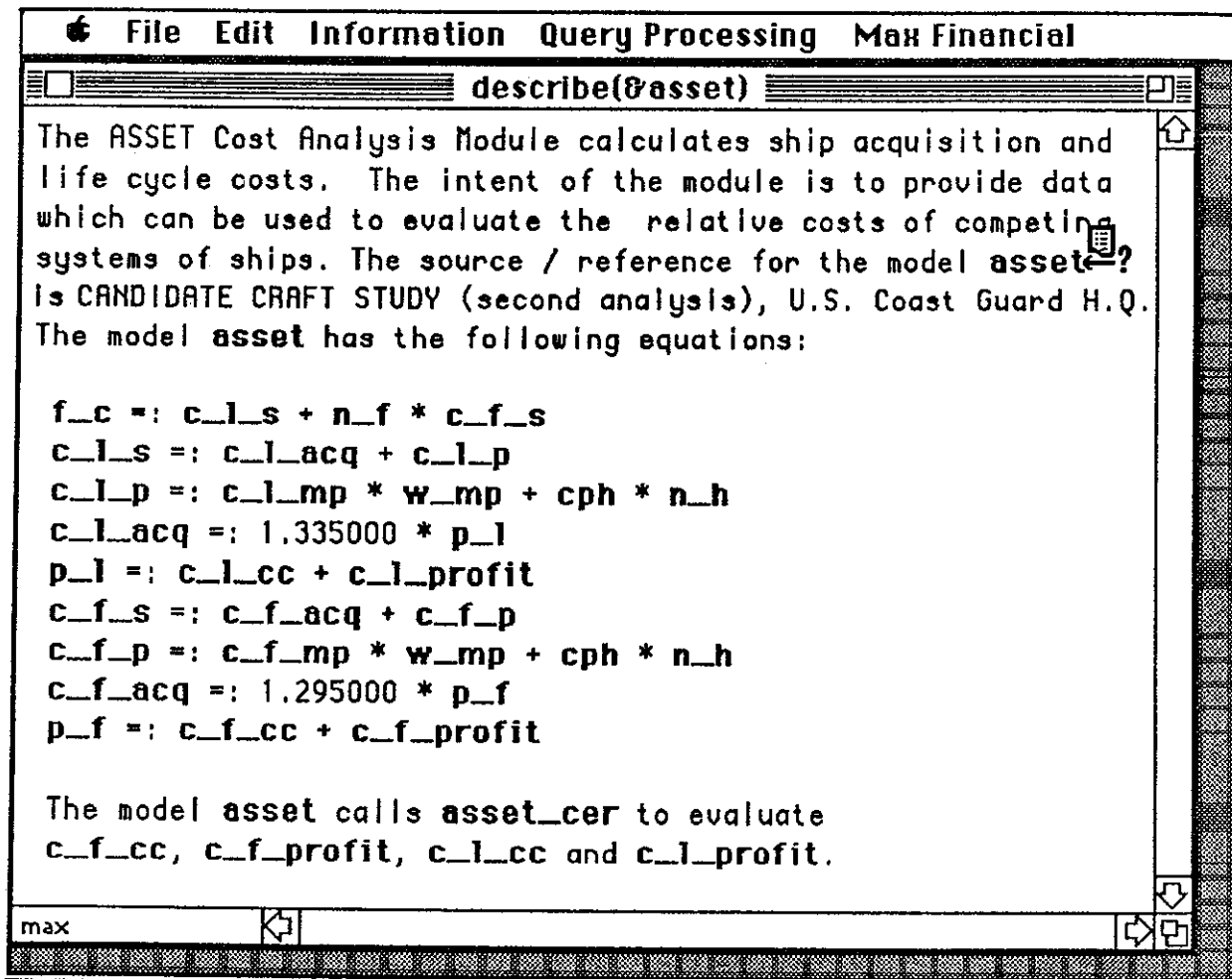
Figure 5. Standard Report Describing the Asset Model
