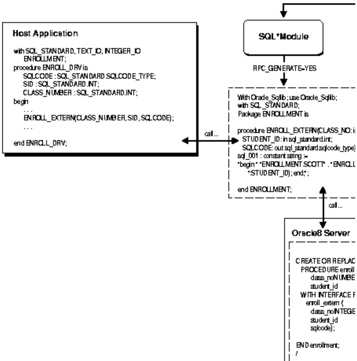
Figure 3-1 Accessing a Stored Procedure
