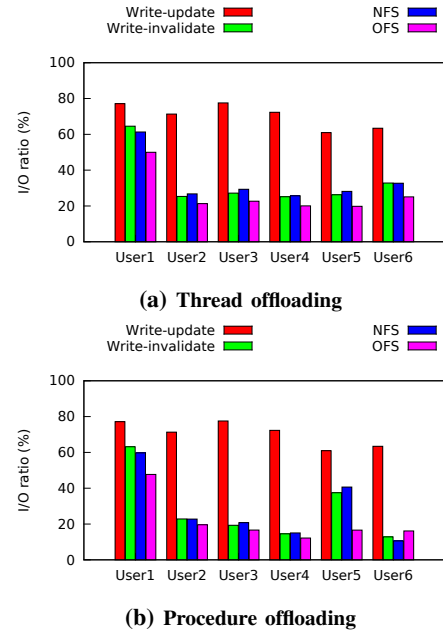
Fig. 10: The ratio between I/O latency and mobile device active time. Four consistency policies are compared: write-update, write-invalidate, close-to-open (NFS), and delayed-update (OFS).
