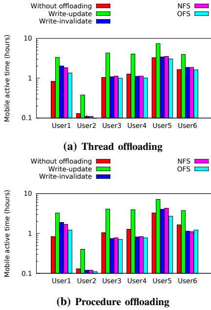
Fig. 9: Total mobile device active time. Four consistency policies are compared: write-update, write-invalidate, close-to-open (NFS), and delayed-update (OFS). In addition, a scenario without offloading is presented. Y axis is in log scale.
