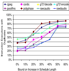
Fig 5: Percentage instruction executions with duplicates
