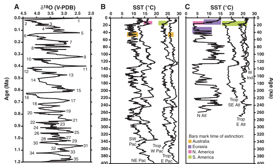
Fig. 2. (A) Oxygen isotope data from benthic foraminifera at North Atlantic Deep-Sea Drilling Program site 607 (81, 82). The isotopic signal ( \delta^{18}\text{O} ) in benthic foraminifera largely reflects variations in continental ice volume, with a smaller effect due to changes in ocean bottom temperatures. Numbers refer to marine isotope stages (81, 82). Most well-constrained extinctions and drops in abundance occurred in stages 2 and 3. V-PDB, Vienna–Pee Dee Belemnite. (B and C) Sea-surface temperature (SST) records from the (B) Pacific and (C) Atlantic and Indian oceans, respectively. Colored bars indicate the time of extinction on nearby continents. The core label, latitude, longitude, type of SST estimate, and source are as follows: northeast Pacific (NE Pac), Ocean Drilling Program (ODP) 1020, 41.00°N, 126.43°W, alkenone (83); tropical east Pacific (Trop E Pac), TR 163-9, 2.26°N, 90.95°W, Mg/Ca (84); tropical west Pacific (Trop W Pac), ODP 806B, 1.32°N, 159.36°E, Mg/Ca (84); southwest Pacific (SW Pac), MD 97-2120, 45.53°S, 174.93°E, Mg/Ca (85); west Indian (W Ind), MD 85674, 3.18°N, 50.43°E, alkenone (86); north Atlantic (N Atl), K 708-1, 50.00°N, 23.73°W, foraminiferal transfer function (average of data reported for August and February) (87); tropical east Atlantic (Trop E Atl), GeoB 1112, 5.77°S, 10.75°W, Mg/Ca (88); and tropical southeast Atlantic (Trop SE Atl), GeoB 10285, 20.10°S, 9.19°E, alkenone (89). All ages in this figure are in calendar years (ky BP), not ^{14}\text{C} years (ky RCBP), using age models in primary publications, except for core K 708-1, where ^{14}\text{C} ages reported in (87) were converted to calendar years with CALIB 98 (90) from 0 to 22,000 ^{14}\text{C} years and with data from (91) for 22,000 to 45,000 ^{14}\text{C} years.
