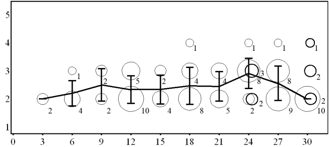
Figure 5: Frequency of occurrence of CCAs and DEC's of sizes 2 through 5 in C1
