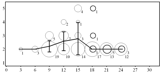
Figure 6: Frequency of occurrence of CCAs and DEC's of sizes 2 through 5 in C2
