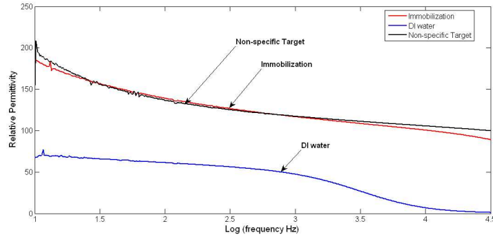
Fig. 5. Dielectric Spectra after the interaction of non-complementary target with the immobilized probe sequence. The slight variation in rel. permittivity value indicates the non-specifically bound oligomers.
