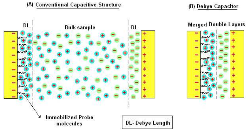
Fig. 2. Comparison between the electrochemical operation of Conventional capacitive sensor and Debye capacitive Sensor
