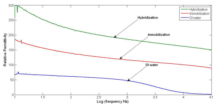
Fig. 4. Dielectric Spectra after hybridization of ( 10\mu\text{M} ) complementary target with the immobilized probe sequence.
