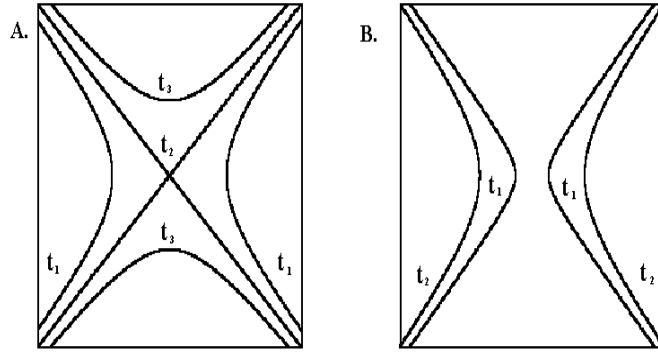
Figure 3 Hyperbolic fronts behaviour
