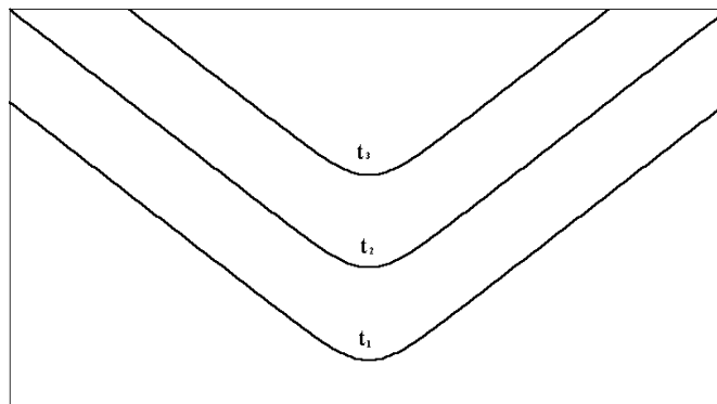
Figure 5 The merging front behaviour
