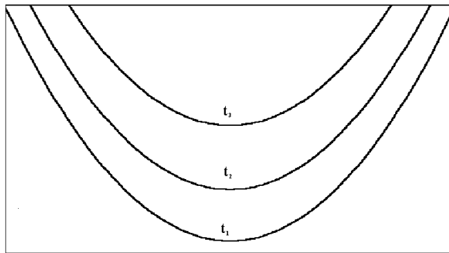
Figure 4 Parabolic front behaviour
