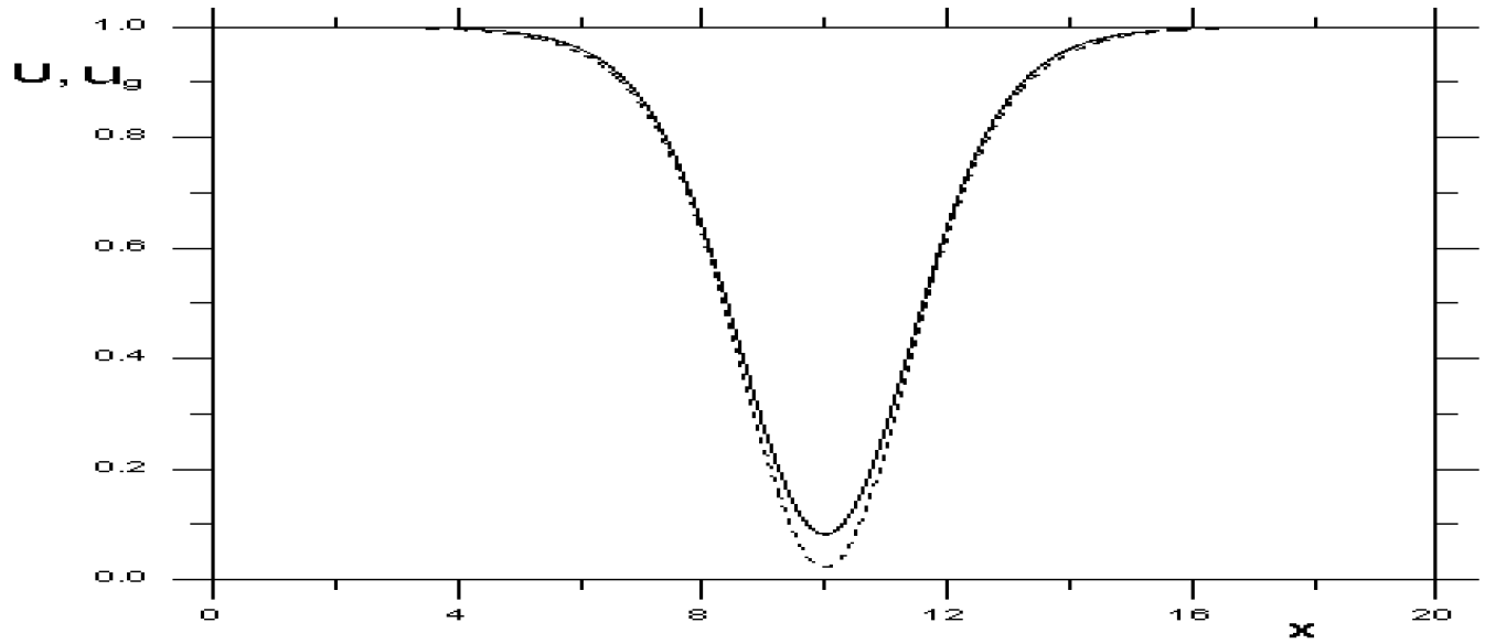
Figure 1 Comparison of the grid solution u_g (dashed line) and approximate solution U , given by the formula (1.11) (solid line) at the moment corresponding to the final stage of the kink — anti kink collision.
