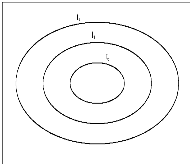
Figure 2 Elliptic front behaviour
