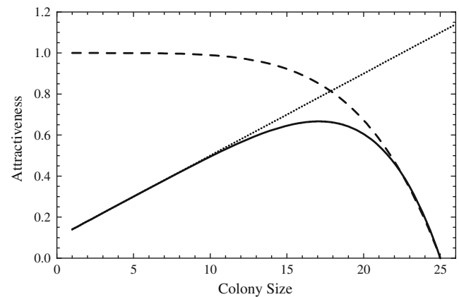
Fig. 3 The attractiveness of a location ( d(N_i) , black line) to an arriving individual as a function of the current colony size at that location. It is the product of the attractiveness based on colonial attraction ( c(N_i) , dotted line) and the attractiveness based on space availability ( I(N_i) , dashed line)
