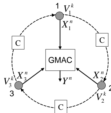
Fig. 1. Three users communicate with an access point over a GMAC, while being connected with each other via a ring of finite-capacity uni-directional links.
