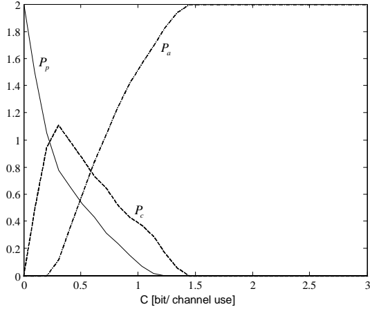
Fig. 3. Optimal power allocation between private message ( P_p ), pair-wise common messages ( P_c ) and network-wise common messages ( P_a ) that maximizes the achievable rate (8) for P = 3 dB.
