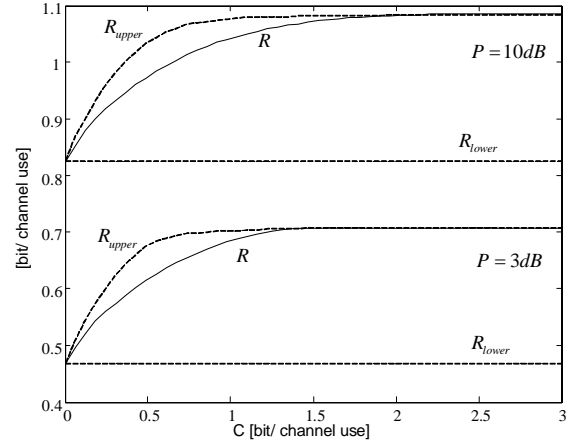
Fig. 2. Achievable rate R (8) and upper bound (5), along with the non-cooperative rate R_{lower} = 1/6 \cdot \log(1 + 3P) , for P = 3 and 10dB with optimal power allocation (evaluated numerically).
