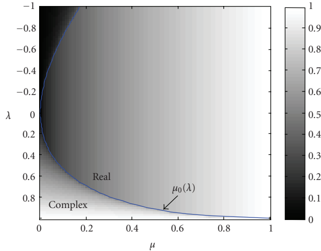
FIGURE 12: Absolute value of the eigenvalue \tilde{\lambda}(\lambda, \mu) (C.3) (with positive sign) of matrix \tilde{\mathbf{A}} (35) versus the eigenvalue a of matrix \mathbf{A} and the pole \mu . Also shown is the threshold value \mu_0(\lambda) (C.5) that discriminates the region where the eigenvalues \tilde{\lambda}(\lambda, \mu) are real or complex conjugate.
