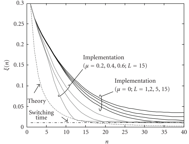
FIGURE 11: Standard deviation of the timing vectors \xi(n) for the synchronization algorithm over a bandlimited Gaussian channel (37) and for the dynamic system (10) (network in Figure 2, SNR = 15 dB, D/d = 2 , \varepsilon = 0.9 , \gamma = 3 , K = 4 ).
