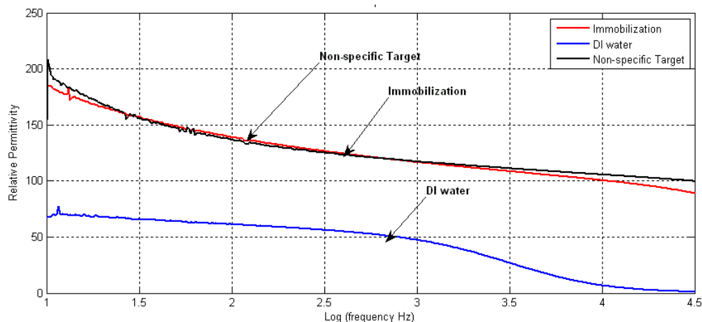
Fig 4b: Dielectric Spectra after the interaction of non-complementary target with the immobilized probe sequence. The slight variation in rel. permittivity value indicates the non-specifically bound oligomers.
