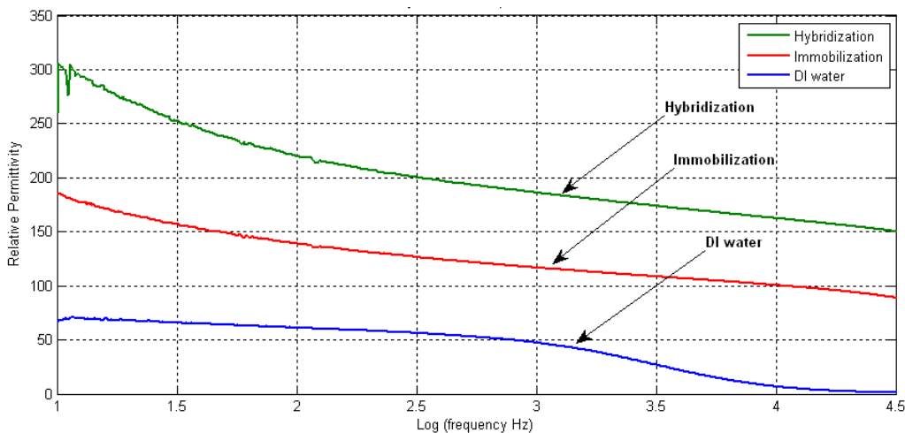
Fig 4a: Dielectric Spectra after hybridization of complementary target with the immobilized probe sequence. The concentration of target used was 10 \mu M.
