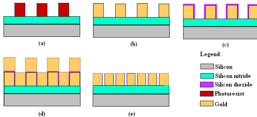
Fig 1. Schematics of the fabrication process flow. a). photo resist spacers are patterned b) gold electrodes formed by sacrificial method c) deposition and patterning of SiO 2 for nanometer spacing d) deposition of gold e) SiO 2 spacer removal
