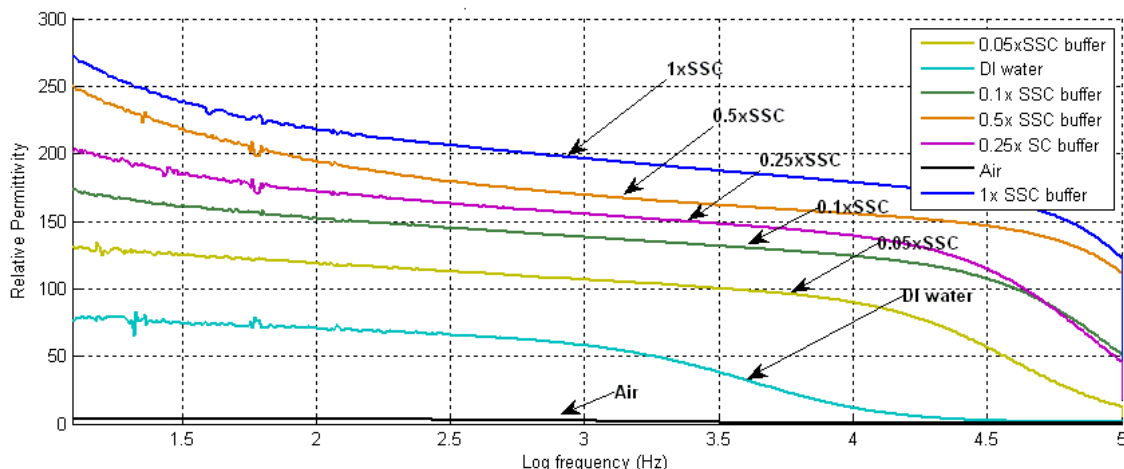
Fig 3: Relative permittivity as a function of frequency for various concentrations of buffer solutions. The measured permittivity increased as the ionic strengths are increased.
