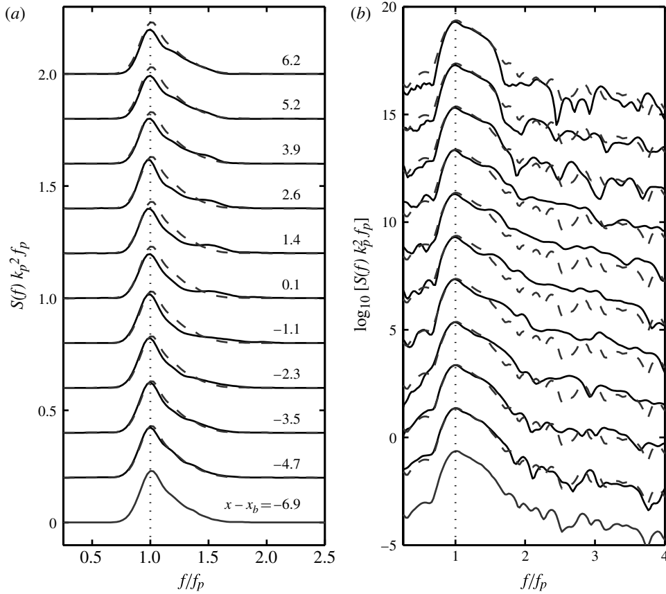
FIGURE 1. Evolution of the wave frequency spectra of a typical non-breaking wave group (W1G1): (a) linear scale and (b) logarithmic scale. Locations of measurements, x - x_b (m), are shown in (a). The dashed lines indicate the reference spectrum measured at the first wave station ( x - x_b = -6.9 m for this case). For clarity, an increment of 0.2 in (a) and 2.0 in (b) is applied along the ordinates to separate the wave spectra at different locations. The vertical dotted lines identify the initial peak frequency (i.e. f/f_p = 1.0 ).
