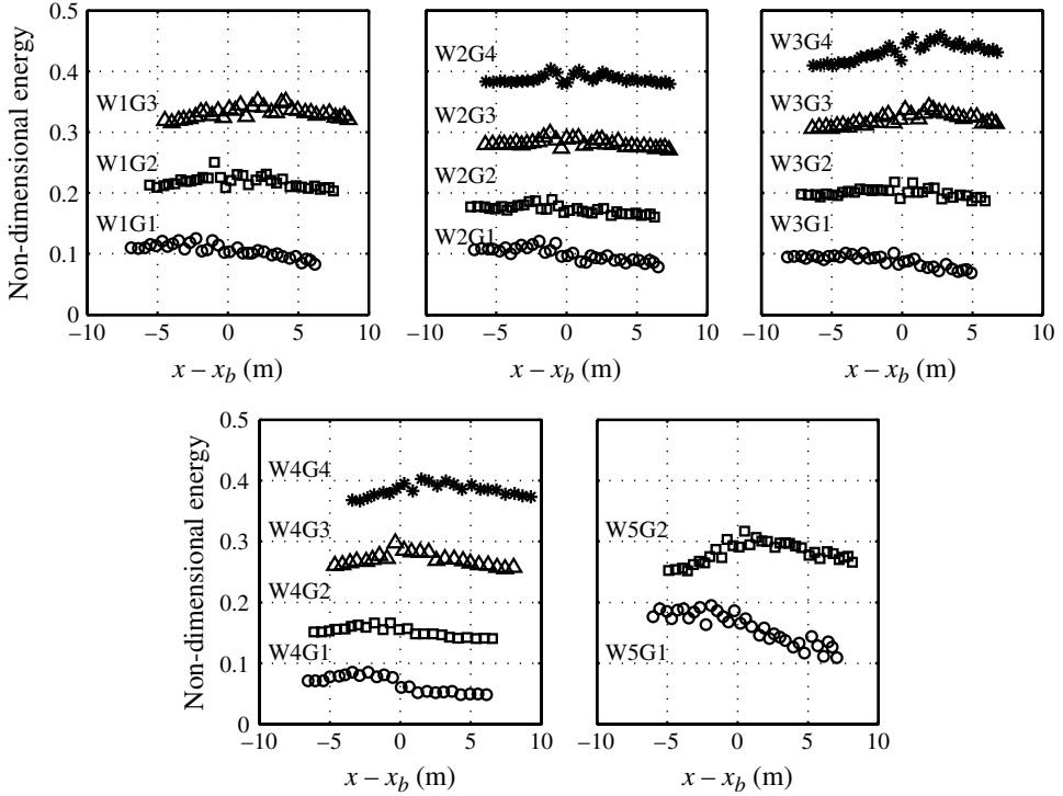
FIGURE 14. Energy in the lower-frequency region ( f/f_p = 0.5 – 0.9 ) as a function of space, E_4(x)/E_{0M} . Here, E_{0M} is the mean of the total energy measured at the first three wave stations. Results for the non-breaking wave groups are represented by the open circles. For clarity, an increase of 0.1 is applied to the ordinate to distinguish wave groups with similar group structure but different gains.
