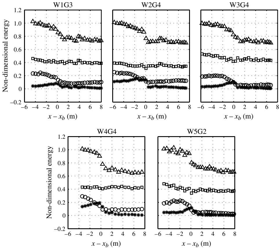
FIGURE 13. Energy levels as a function of space for the breaking wave groups (shown only for the most violent breaker among wave groups with similar structures). Triangles, E_0(x)/E_{0M} ; squares, E_1(x)/E_{0M} ; circles, E_2(x)/E_{0M} ; asterisks, E_3(x)/E_{0M} . Here, E_0(x) are the total energy ( f/f_p < 4 ); E_1(x) the energy near the spectral peak region; E_2(x) the energy in the above-peak region; and E_3(x) the energy in the higher-frequency region; E_{0M} is the mean of the total energy measured at the first three wave stations.
