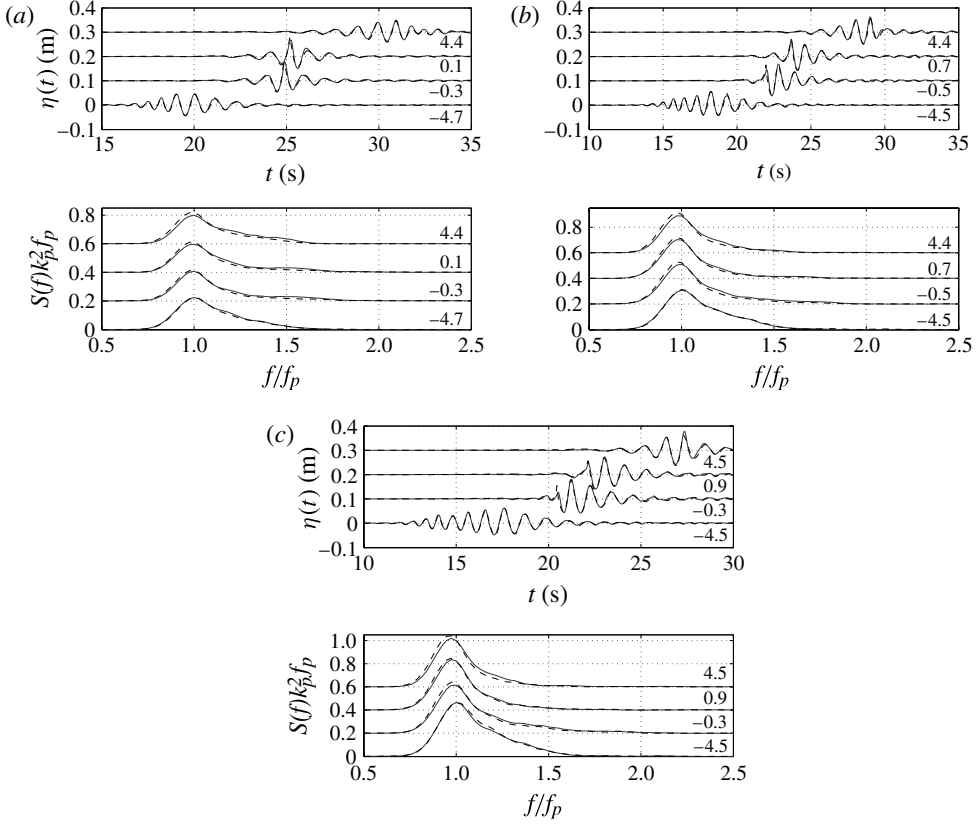
FIGURE 15. Comparisons between the experimental results of the surface elevation and the corresponding wave frequency spectra for a typical non-breaking wave group (W1G1) and two typical breaking wave groups (W1G2 and W1G3). Solid curves represent the experimental results and dashed curves are the numerical results. Locations relative to the wave focusing/breaking point, x - x_b (m), are indicated to the right of each set of graphs. For clarity, increments of 0.1 and 0.2 are applied to the ordinates for the surface elevation and the wave spectra, respectively: (a) W1G1; (b) W1G2; (c) W1G3.
