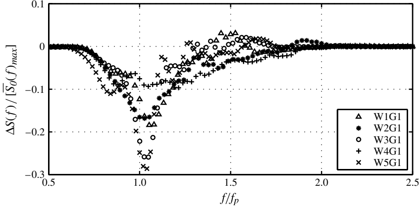
FIGURE 4. Spectral distribution of the non-breaking dissipation. \overline{S}_{0max} indicates the peak of the mean wave spectrum determined with the first three wave station measurements.
