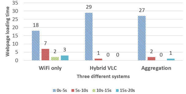
Fig. 14. Statistic of yahoo homepage loading time
