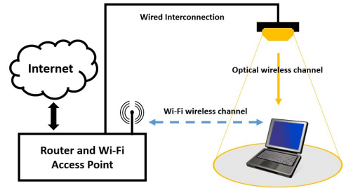
Fig. 2. Proposed hybrid WiFi and VLC network model
