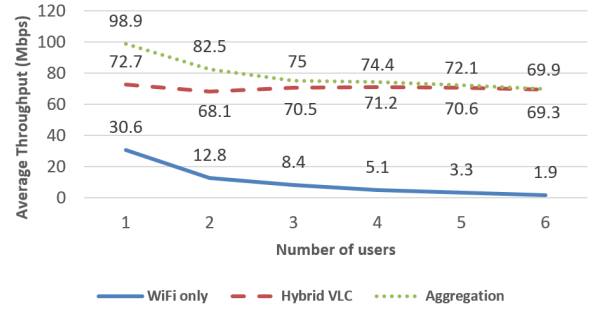
Fig. 12. Throughput vs. Number of users
