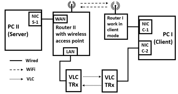
Fig. 5. Aggregated system architecture
