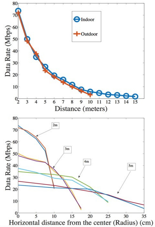
Fig. 10. Throughput vs. vertical and horizontal distance between VLC transceivers
