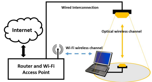
Fig. 3. Proposed aggregated WiFi and VLC network model
