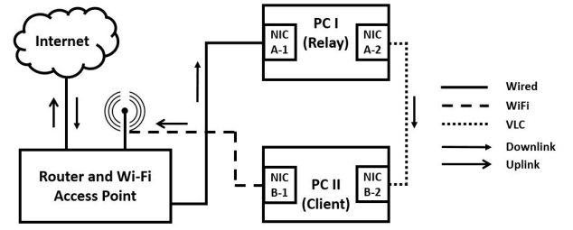
Fig. 4. Hybrid system architecture
