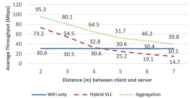
Fig. 15. Throughput vs. Distance between tx and rx
