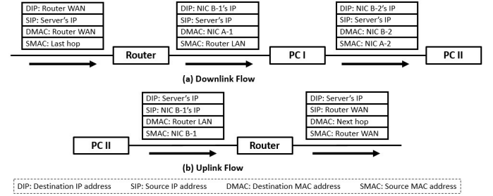
Fig. 6. Flow of MAC and IP headers of packets between server and client, a) downlink flow and b) uplink flow
