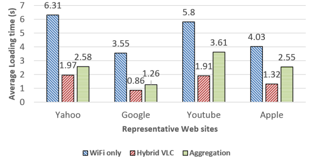
Fig. 13. Loading time in web browsing
