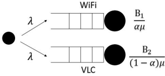
Fig. 7. Queuing model representing the aggregated system model
