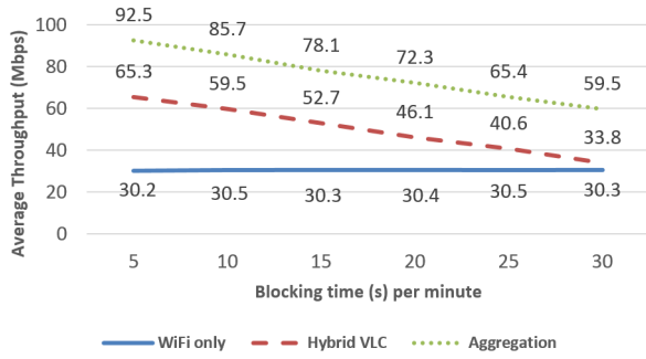
Fig. 16. Throughput vs. Block duration
