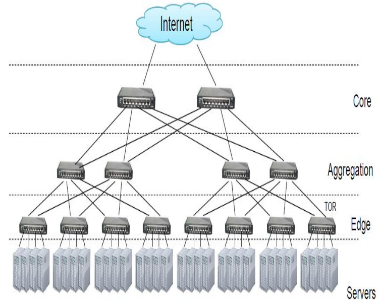
Figure 11: Network topology
