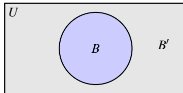
Figure 1.5: Venn diagram : B'
