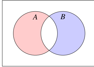
Figure 1.8: Venn diagram : A \oplus B
