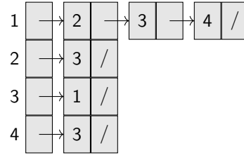
Figure 10.12: Its adjacency list A
