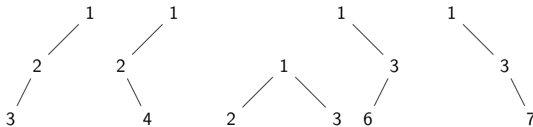
Figure 10.4: (Rooted) binary trees n = 3 .
