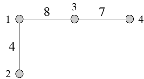
Figure 10.26: Step 1 of Kruskal's algorithm
