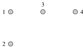
Figure 10.30: Prim's Step 0: X = \{4\} .
