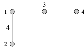
Figure 10.26: Step 1 of Kruskal's algorithm
