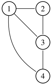
Figure 10.13: An undirected graph
