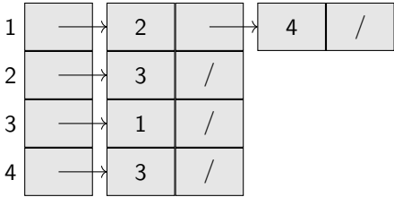
Figure 10.18: Its adjacency list A
