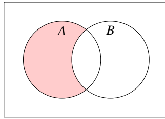
Figure 1.6: Venn diagram : A - B
