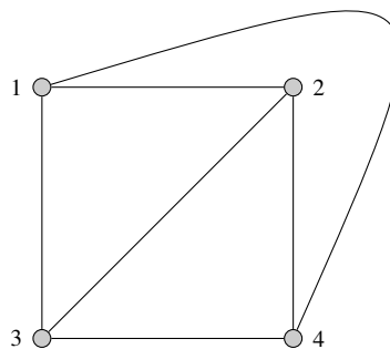
Figure 10.8: A K_4 graph: planarity form
