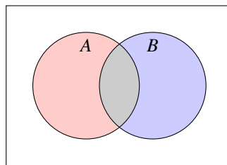
Figure 1.2: Venn diagram : A \cap B
