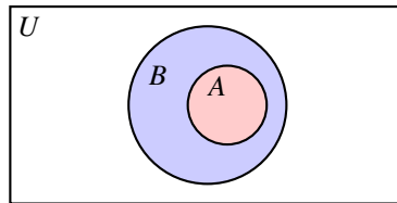
Figure 1.1: Venn diagram : A \subseteq B
