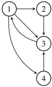
Figure 10.10: A directed graph
