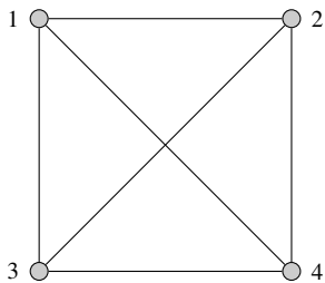
Figure 10.7: A K_4 graph: traditional view
