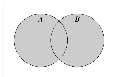
Figure 1.4: Venn diagram : A \cup B
