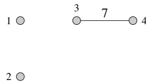
Figure 10.31: Prim's Step 1: X = \{4, 3\} .
