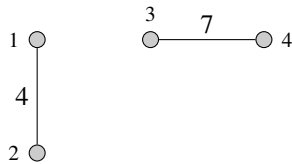
Figure 10.25: Step 0 of Kruskal's algorithm
