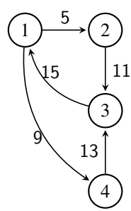
Figure 10.16: A weighed directed graph
