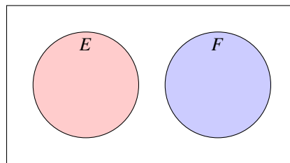
Figure 1.3: Venn diagram : E \cap F = \emptyset
