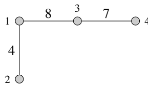
Figure 10.33: Prim's Step 3: X = \{4, 3, 1, 2\} .
