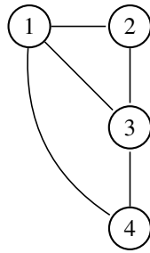
Figure 10.2: An undirected graph
