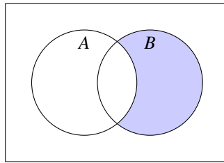
Figure 1.7: Venn diagram : B - A
