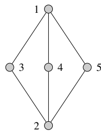
Figure 10.6: A K_{2,3} graph: planarity form
