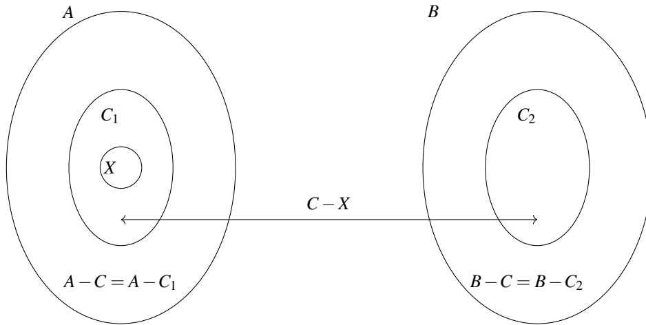
Figure 10.9: Venn diagrams for sets of Theorem 10.18
