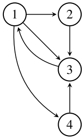
Figure 10.1: A directed graph
