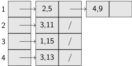
Figure 10.20: Its weight list W
