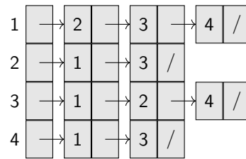
Figure 10.15: Its adjacency list A
