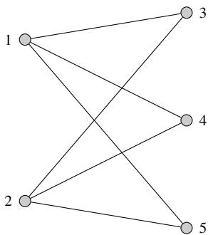
Figure 10.5: A K_{2,3} graph: traditional view
