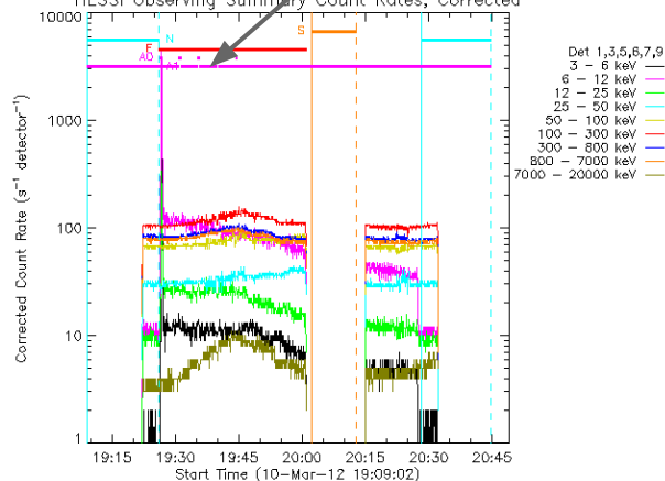
HESSI Observing Summary Count Rates, Corrected
