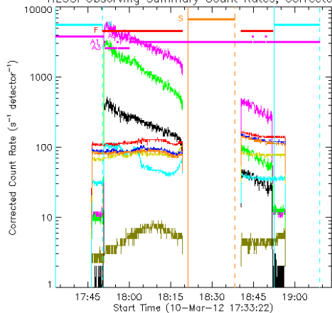
HESSI Observing Summary Count Rates, Corrected
