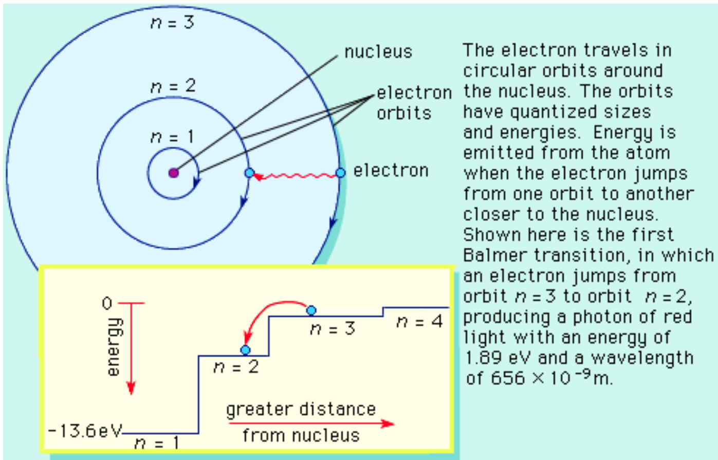
An hydrogen atom
