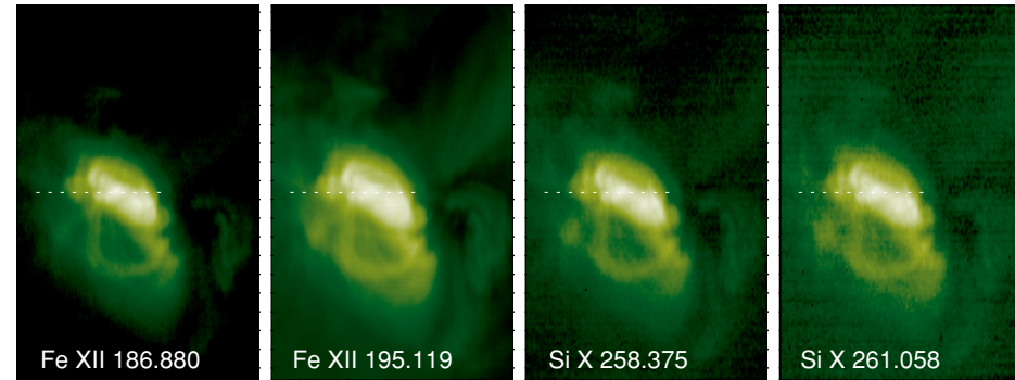
Observation from Hinode/EIS
