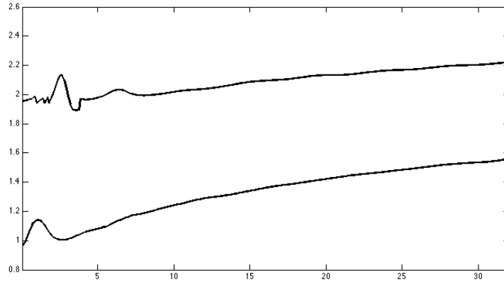
Figure 4: Plots of the decimal logarithms of the condition numbers of the discretizations of the formulations DCFIE-RC(0,1) using the regularizing operators S_{ik/2} and \eta = 1 as functions of the wave number k for the boomerang geometries. We chose 320 wave numbers k = 0.1, 0.2, \dots, 32 and 128 unknown for each case, p = 4 in the change of variables formula (50) for each boomerang geometry. The curve on the bottom corresponds to the case \alpha = 1/2 and the curve on the top corresponds to the case \alpha = 1/6 .
