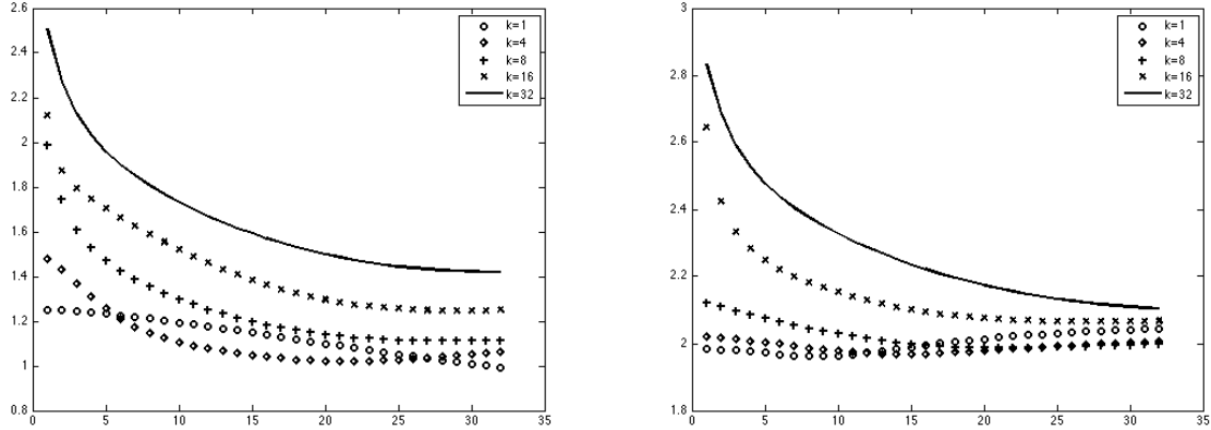
Figure 3: Plots of the decimal logarithms of the condition numbers of the discretizations of the formulations DCFIE-RC(0,1) using the regularizing operators S_{ik/2} as functions of the wave number k and the coupling parameter \eta for the boomerang geometries with \alpha = 1/2 (left) and \alpha = 1/6 (right). The results shown correspond to problems having 128 unknowns, and wave numbers k = 1, 4, 8, 16, 32 and 32 coupling parameters for each formulation: \eta = j/16 , j = 1, 2, \dots, 32 .
