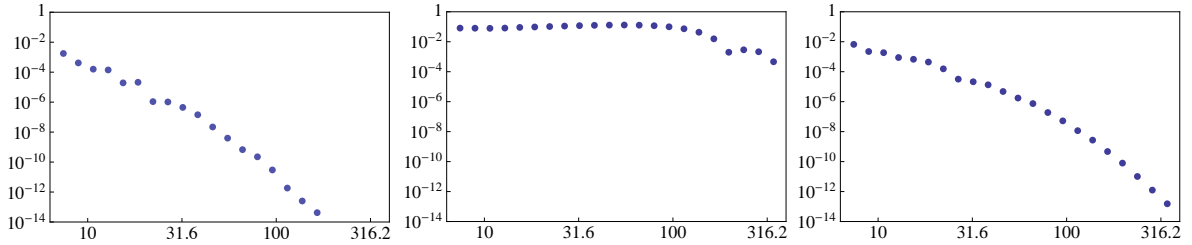
Figure 2: These plots are similar to those in Fig. 1 except that the Bloch wavevector is (\kappa_1 = 0.4, \kappa_2 = -0.3) , and the frequencies are k = 0.3, 0.93, 1.1 . There is a Wood frequency at \sim 0.921954 .
