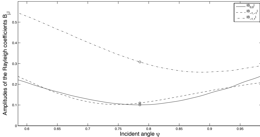
Figure 3: Plot of the amplitudes of the Rayleigh modes |B_{0,0}| , |B_{-1,-1}| , and |B_{-1,1}| for the wavenumber k = 2\sqrt{2}\pi as a function of the azimuthal angle \psi around the value \psi_0 = \pi/4 . We took \phi = 0 in all of these experiments. For incidence angles \psi_0 = \pi/4 and \phi = 0 , the value k = 2\sqrt{2}\pi is a Wood anomaly since \gamma_{0,1} = 0 . We considered 60 values of the incidence angle \psi in a small neighborhood of \psi_0 = \pi/4 . The values of the Rayleigh amplitudes at the Wood frequency corresponding to \psi_0 = \pi/4 are depicted by \circ . For each scattering experiment we computed the conservation of energy error \epsilon and the magnitude of those did not exceed 2%.
