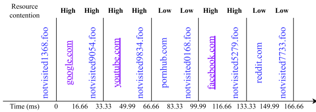
Fig. 1. Method A of history sniffing attacks: two calls to the requestAnimationFrame API. We use the standard color convention used by browsers to denote visited/unvisited URLs: blue for unvisited links and purple for visited links .
