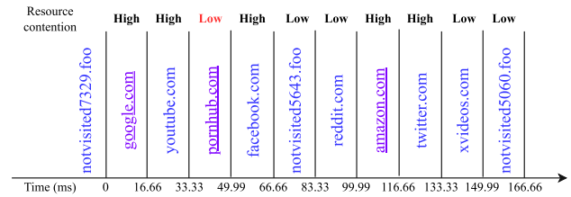
Fig. 2. Method B of history sniffing attacks: one call to the requestAnimationFrame API. We use the standard color convention used by browsers to denote visited/unvisited URLs: blue for unvisited links and purple for visited links .
