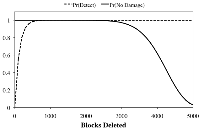
Figure 4: Probability of an attack failing because either no data was damaged or the audit process detected deleted blocks.
