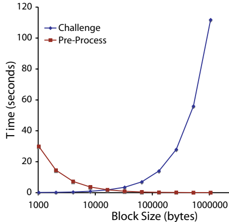
Figure 6: E-PDP pre-processing vs. challenge trade-offs with block size for a 1 MB file.
