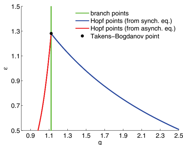
Figure 7. Two-parameter bifurcation diagram indicating a TB singularity in the three-cell reduction (1.4) at g = 1.123 , \varepsilon = 1.281 . In these computations we set w^* = 0.25 , \beta^* = 1.5 , and I^* = 1 and calculate z^* = 0.763 and u^* = 0.934 .
