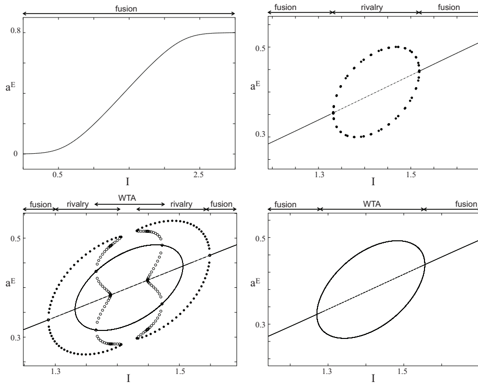
Figure 10. Bifurcation diagrams in the original system (1.2) corresponding to the different paths through the \mu_1\mu_2 plane shown in Figure 9. In all panels, I is varied while \beta = \beta^* = 1 and \varepsilon = \varepsilon^* = \frac{2}{3} . Top left: \alpha = \alpha_0^* = 0.157 , g = g^* = 0.463 (path 1). Top right: \alpha = 1.1\alpha_0^* , g = 1.05g^* (path 2). Bottom left: \alpha = 1.2\alpha_0^* , g = 1.05g^* (path 3). Bottom right: \alpha = \alpha_0^* , g = 0.95g^* (path 4).
