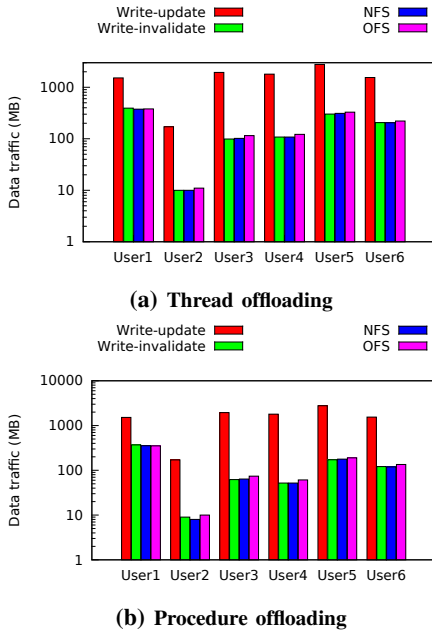
Fig. 6: The amount of network overhead incurred by the workloads. Four consistency policies are compared: write-update, write-invalidate, close-to-open (NFS), and delayed-update (OFS). The Y axis is in log scale.
