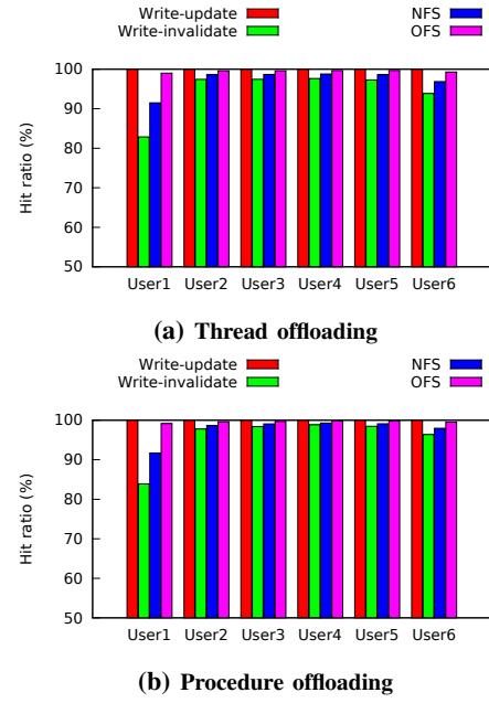
Fig. 8: Block buffer hit ratios. Four consistency policies are compared: write-update, write-invalidate, close-to-open (NFS), and delayed-update (OFS).
