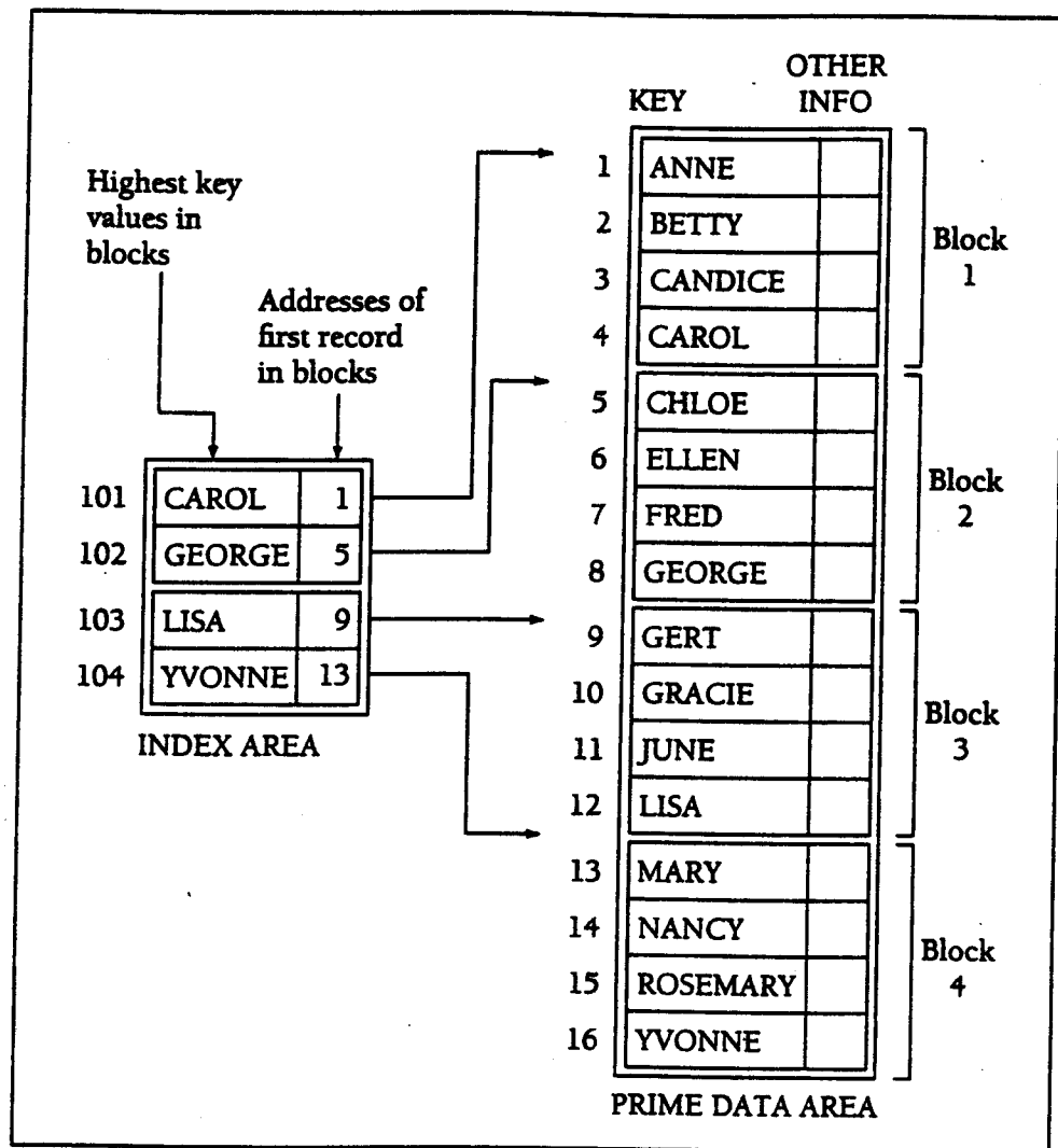
Figure 2 Indexed Sequential Organization with a Single-Level Index
