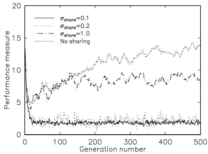
Figure 16: Effect of varying \sigma_{share} values is shown for problem F1.
