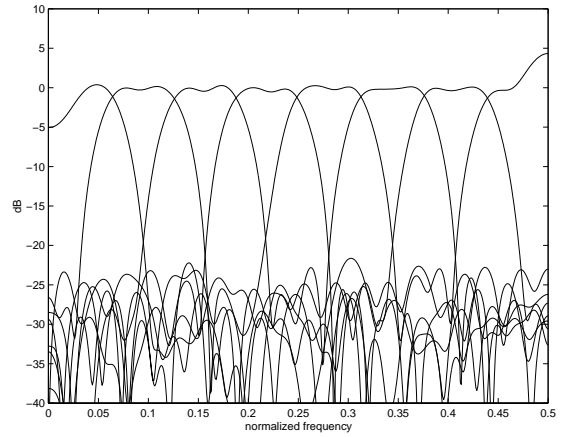
Figure 3: Normalized frequency response of low-delay integer-modulated filter bank with M = 8 subbands, D = 15 , and filter length L = 44 .
