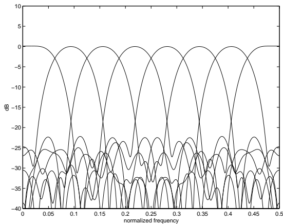
Figure 2: Normalized frequency response of integer-modulated paraunitary filter bank with M = 8 subbands and filter length L = 32 .
