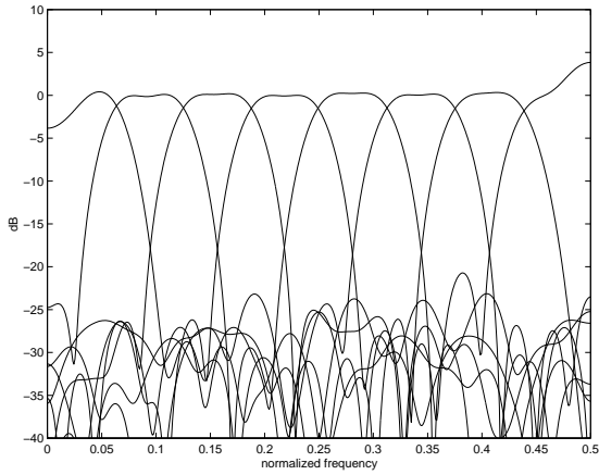
Figure 1: Normalized frequency response of low-delay integer-modulated filter bank with M = 8 subbands, D = 15 , filter length L = 32 , and coefficients from Table 1.
