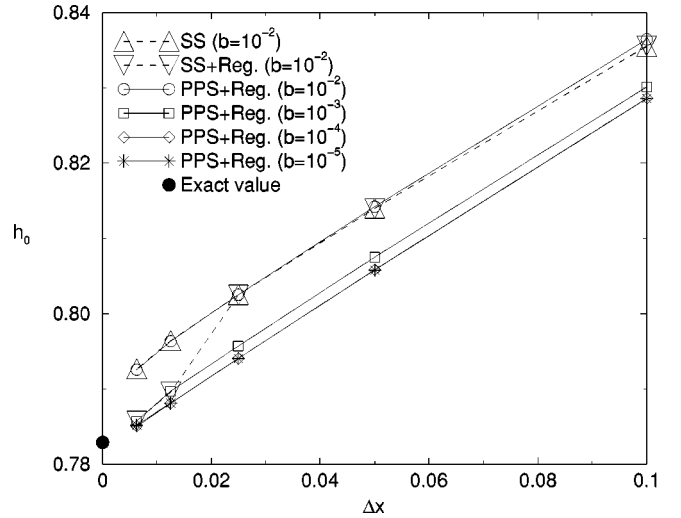
FIG. 3. Thickness h_0 of the planar drop for n=1 ( t=0.02 ) as a function of \Delta x with several values of b , under different schemes. For b=10^{-3} , \mathcal{SS} leads to negative results for the film thickness (not shown).
