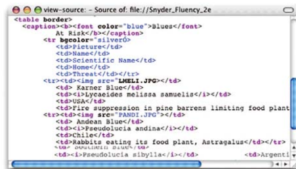
Figure 7.8 The Source View displayed by the Firefox browser for the start of the table.
