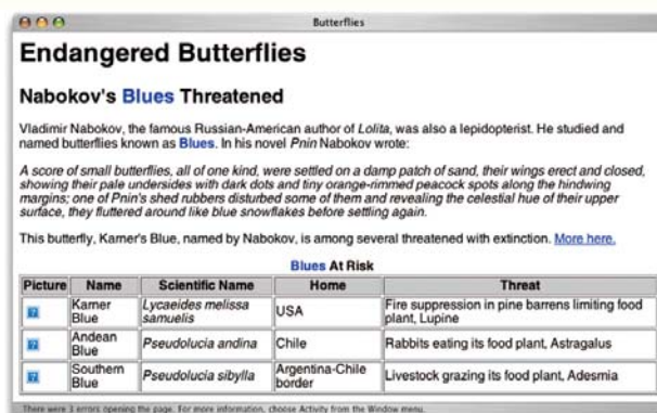
Figure 7.9 The Butterflies page after correcting the heading color.
