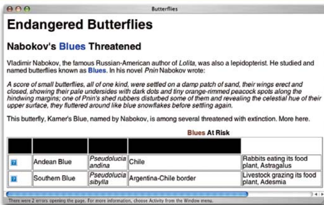
Figure 7.3 The Butterflies page displayed by the Safari browser.
