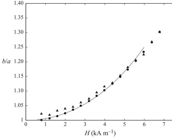
FIGURE 16. Comparison of direct numerical simulations (●) with experimental data (▲) and with the theory discussed in § 3.2 (—) for low applied fields. Drop shapes are shown in figure 17.
