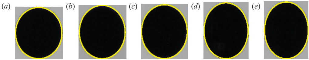
FIGURE 17. (Colour online) Numerically simulated drop equilibrium shapes are highlighted and superimposed over experimentally obtained images. The values for the applied magnetic field (0, 0, H_o) kA m -1 are H_o = (a) 3.978, (b) 4.774, (c) 5.172, (d) 6.366 and (e) 6.764.
