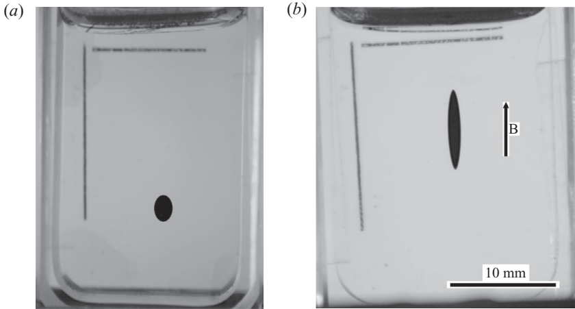
FIGURE 2. Experimental photographs of the deformation of a PDMS ferrofluid drop in a viscous medium under applied uniform magnetic fields. (a) H_o = 6.38 \text{ kA m}^{-1} and (b) 638.21 \text{ kA m}^{-1} . Images were collected using the equipment shown in figure 11 (Tyler 2008).
