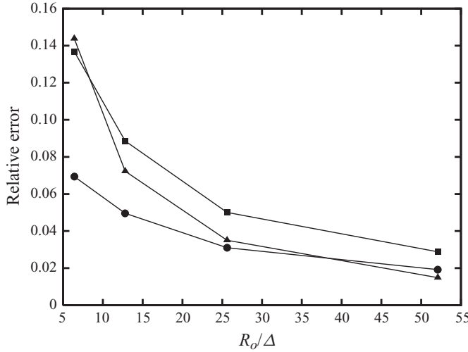
FIGURE 6. Relative error, |[[p]]_{\text{exact}} - [[p]]_{\text{computed}}| / |[[p]]_{\text{exact}}| , in the calculated pressure jump at \theta = 90^\circ (▲), 45^\circ (●) and 0^\circ (■) as a function of spatial refinement.
