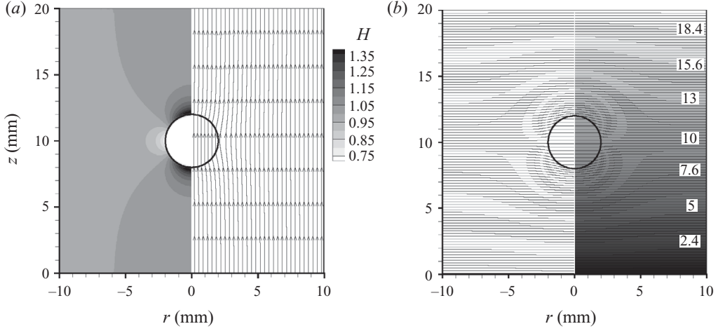
FIGURE 5. (a) Contours of the magnetic field ( \text{kA m}^{-1} ) on the left and magnetic field lines on the right and (b) magnetic field potential (A) are plotted in the presence of a ferrofluid droplet in a non-magnetizable medium. \chi = 1 .
