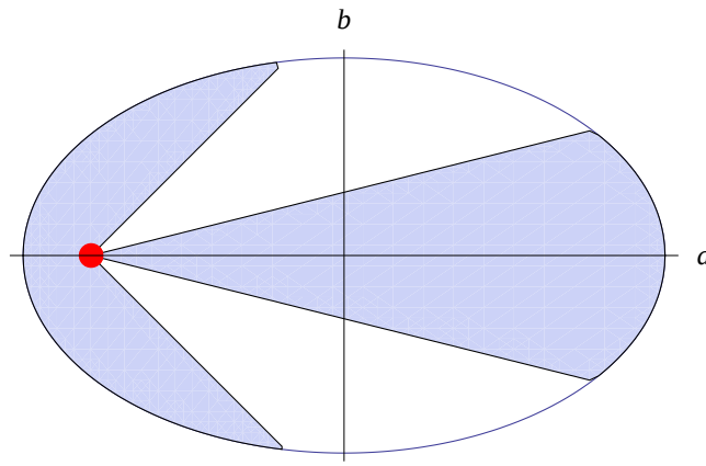
FIG. 39: The ellipse and Kepler's Law's:
