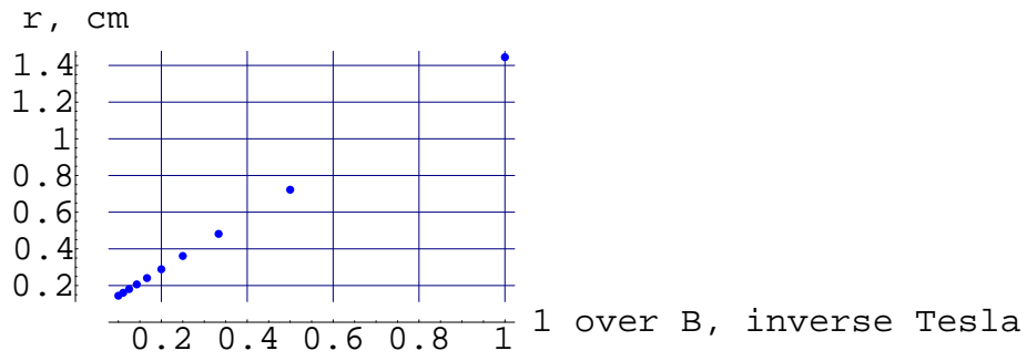
Figure 1: Radius of revolution as a function of inverse magnetic field for a particle accelerated through a potential difference of 10 kV.
