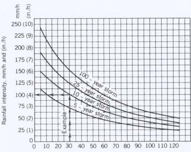
FIGURE 3.6 Typical rainfall intensity–duration–frequency curves. Curves like these are prepared from rainfall statistics by the U.S. National Climatic Data Center.
