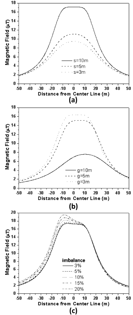
Fig. 4. Profile of the resulting magnetic field from the 500-kV transmission-line model in Fig. 3(a) at midspan. (a) Simulated with different sagging ( s ). (b) Simulated with different galloping ( g ). (c) Simulated with different current imbalance. The distance from the center line is along the x -direction.
