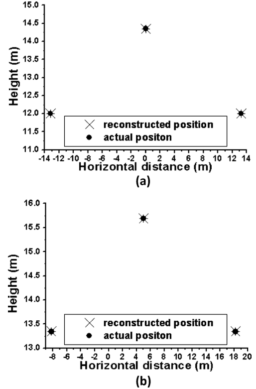
Fig. 8. Actual and reconstructed positions of phase conductors when (a) conductor sagging is 10 m, and (b) line galloping is 5 m with 10-m sag.
