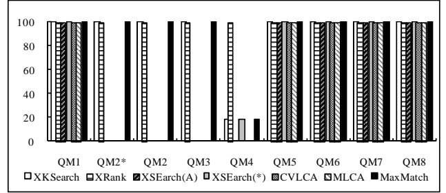
(b) Recall
