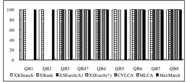
(b) Recall
